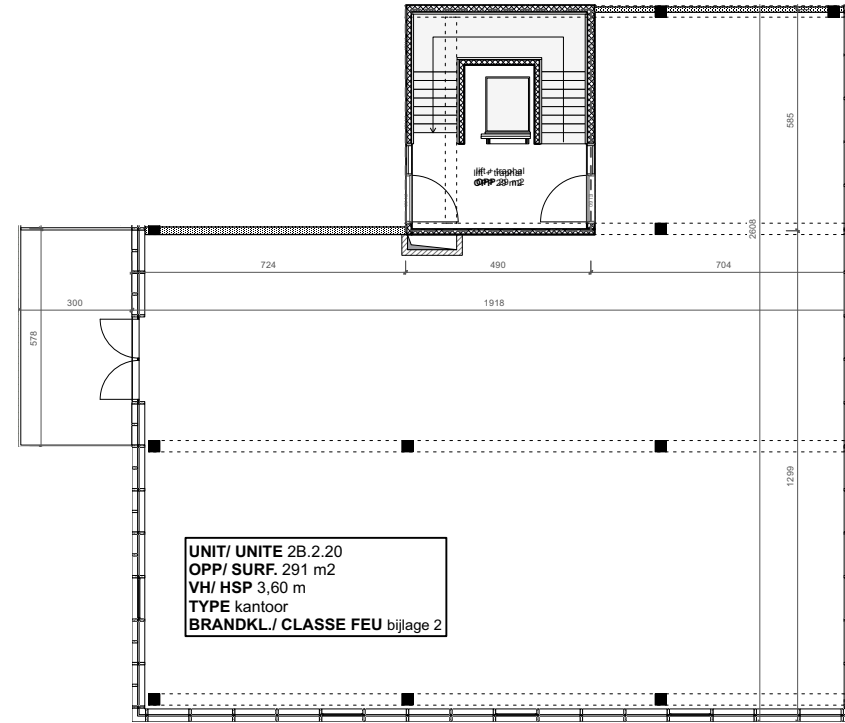
PLAN +1 - unit 2B.2.20
