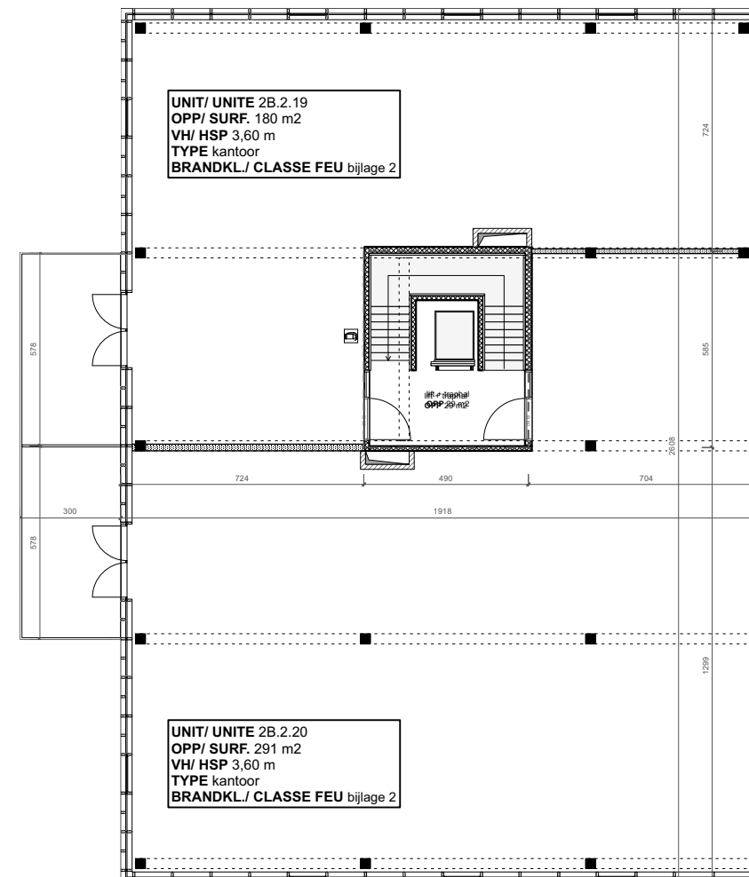
PLAN +1 - unit 2B.2.19 en 2B.2.20
